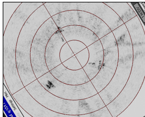
Fig. 7. Radial-pattern sonar image (image 040909).
