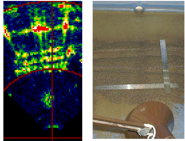
Fig. 3. Imagenex sonar image (left) of test ripples (about 1-2 cm height, about 10 cm length) in tank. Red range rings are 1 m increments. Three sand ripples are shown starting at 1 m range (first red ring).
